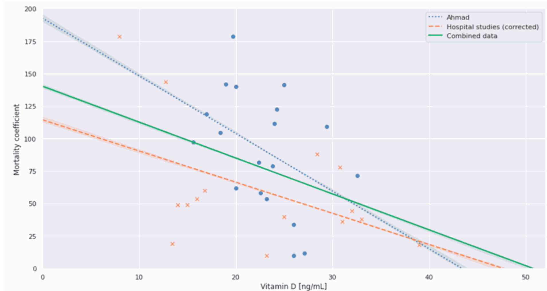
Figure 5. Scatter plot and OLS regressions of the individual and combined datasets.
